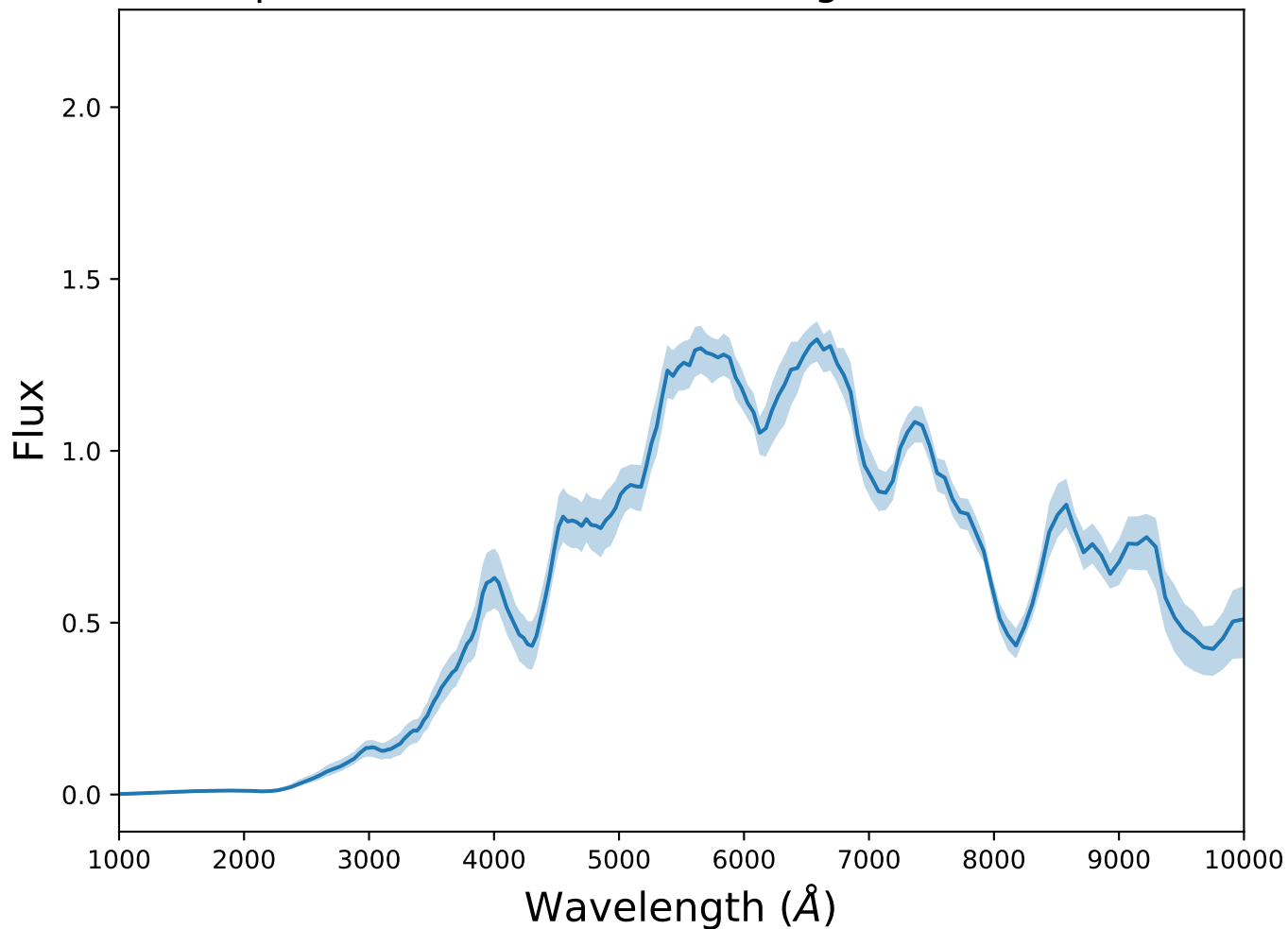
Spectrum 4 for transient 91bg-like at z=1.65
